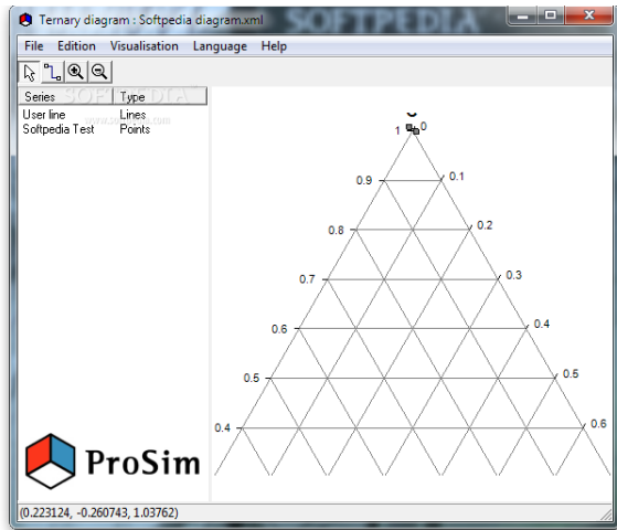
Simulis® Thermodynamics
